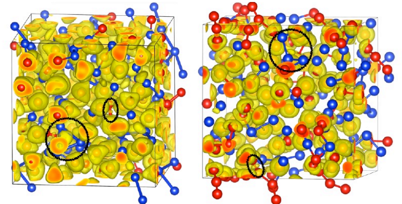
Electron Localization Function in silica at extreme conditions
